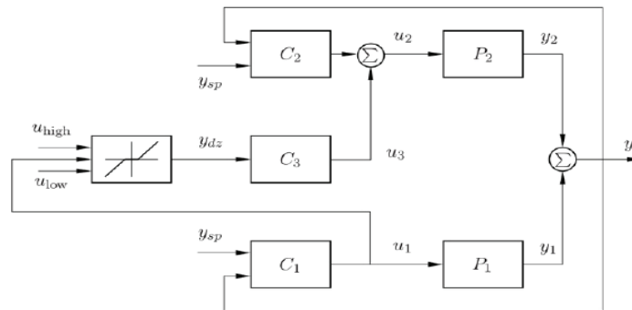
The feedforward mid-ranging control structure
